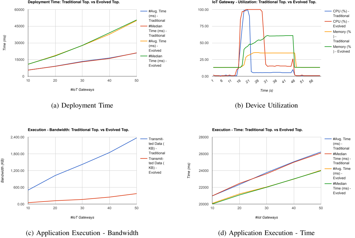
Fig. 4: Evaluation Results
